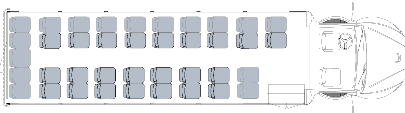
Model 375 - 39 Passenger plus driver & co-pilot
