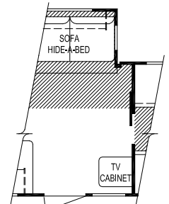
Option Front Entry (Model 386)
