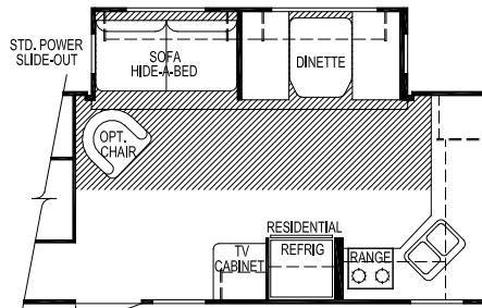
Opt. Front Entry (Model 380)
