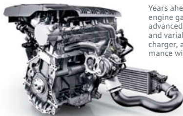
.14 - 2.0 TFSI Turbocharged Engine
