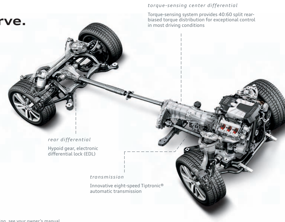
torque-sensing center differential
