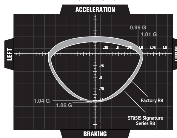
TRACTION CIRCLE
