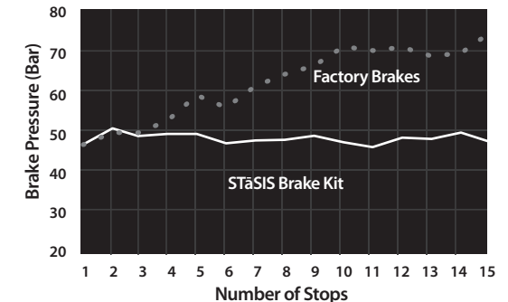
HIGH-SPEED FADE TEST OVER CONSECUTIVE STOPS MAINTAINING 0.7 G
