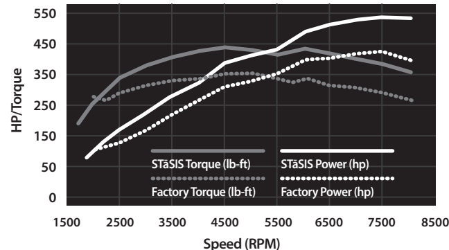
HORSEPOWER/TORQUE GAINS
