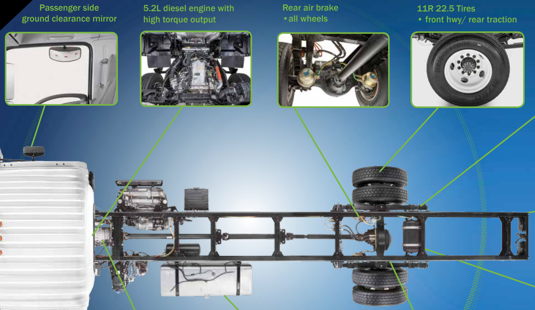
Rear Bolted Suspension
