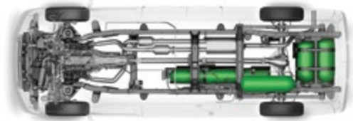
FOUR-TANK SYSTEM
