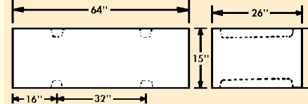
98 GALLON POLY TANK, NO FITTINGS 23729 98 Gal. Tank #W1078 1
