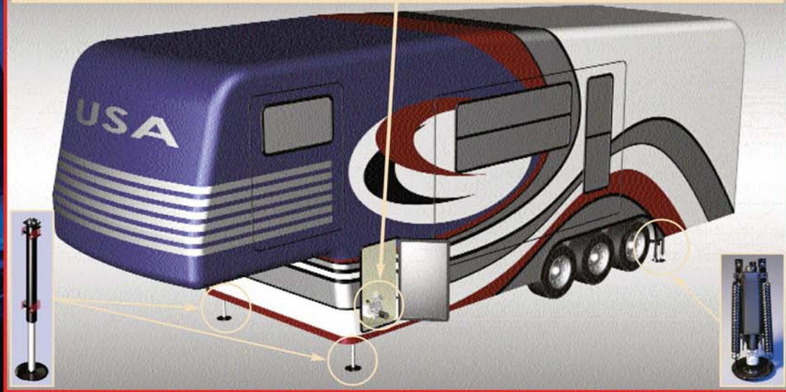
Hand pump with hydraulic switches (no electric power is required)
