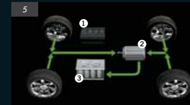
FIG. 5: REGENERATIVE BRAKING
