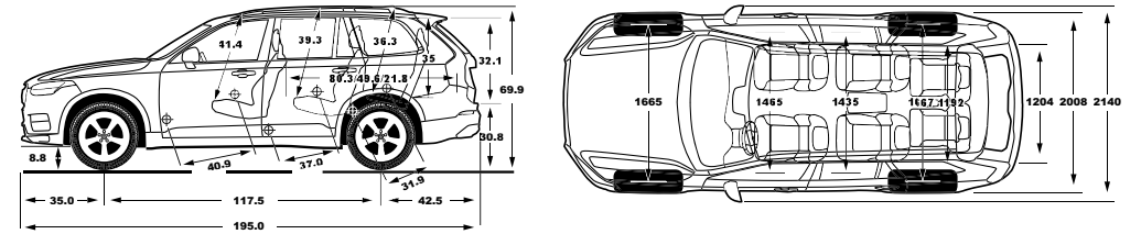
6-SEAT VERSION
